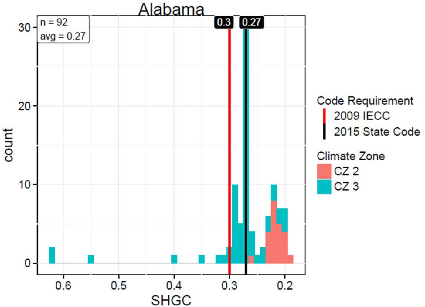
Figure 3.2. Window SHGC
