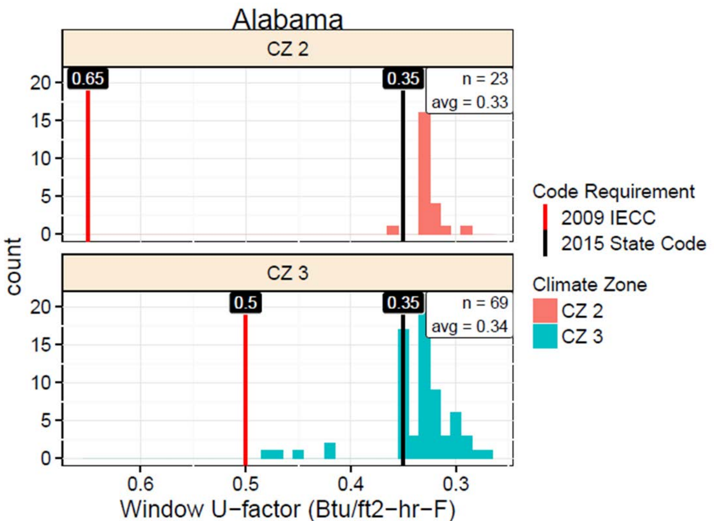
Figure 3.3. Window U-Factor
