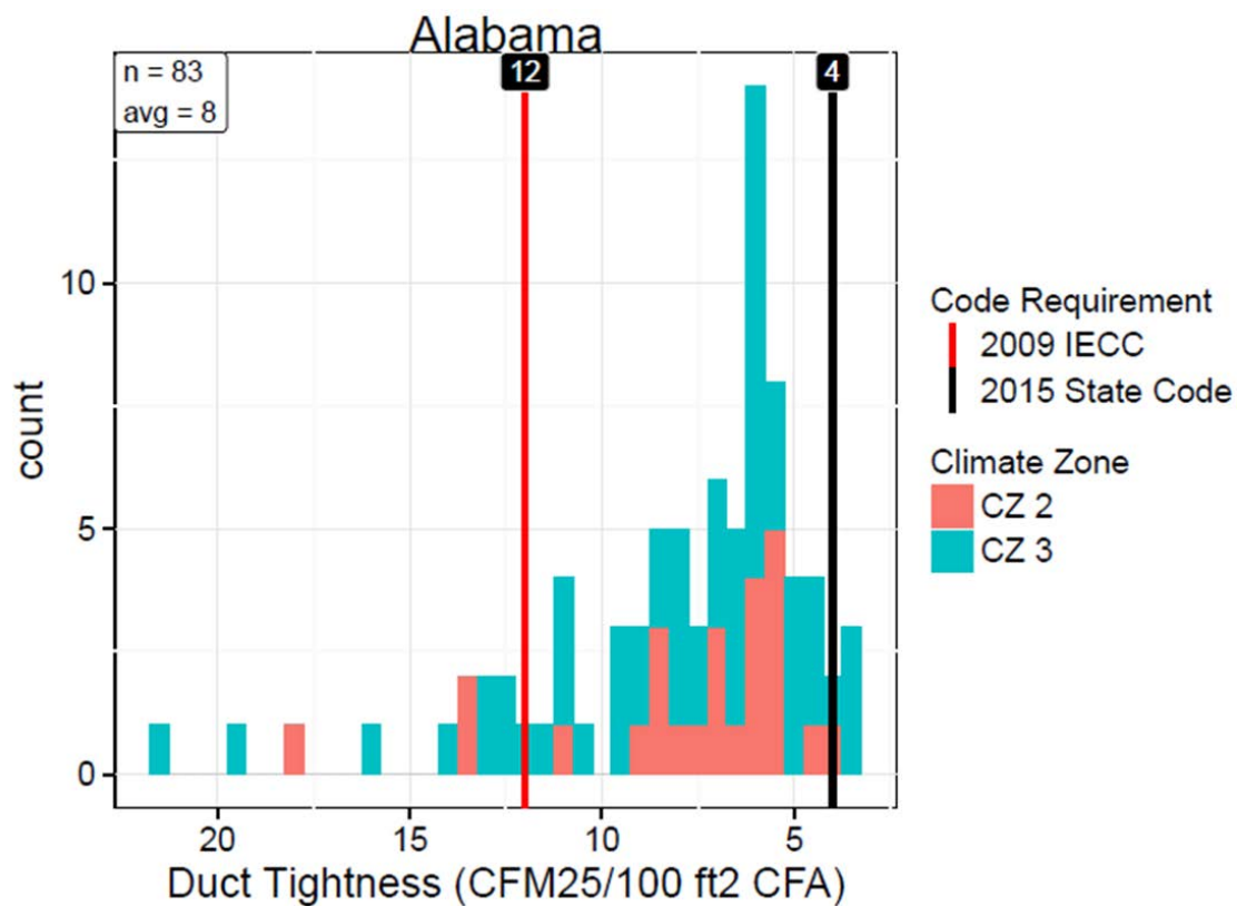
Figure 3.7. Duct Tightness (CFM25/100ft² CFA)
